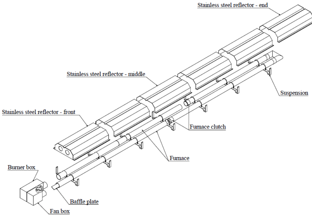
Fig. 3 Infrared heater KM-U with length 10 and 12 m
