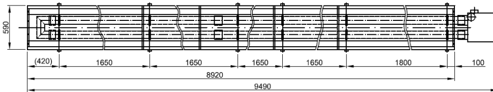
KM 45-U-10m
