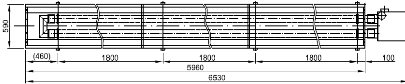
KM 22,5-U-8m
