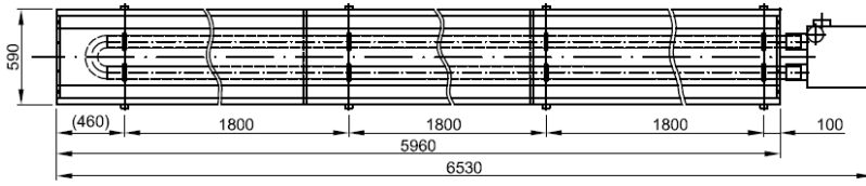
KM 22,5-U-6m
