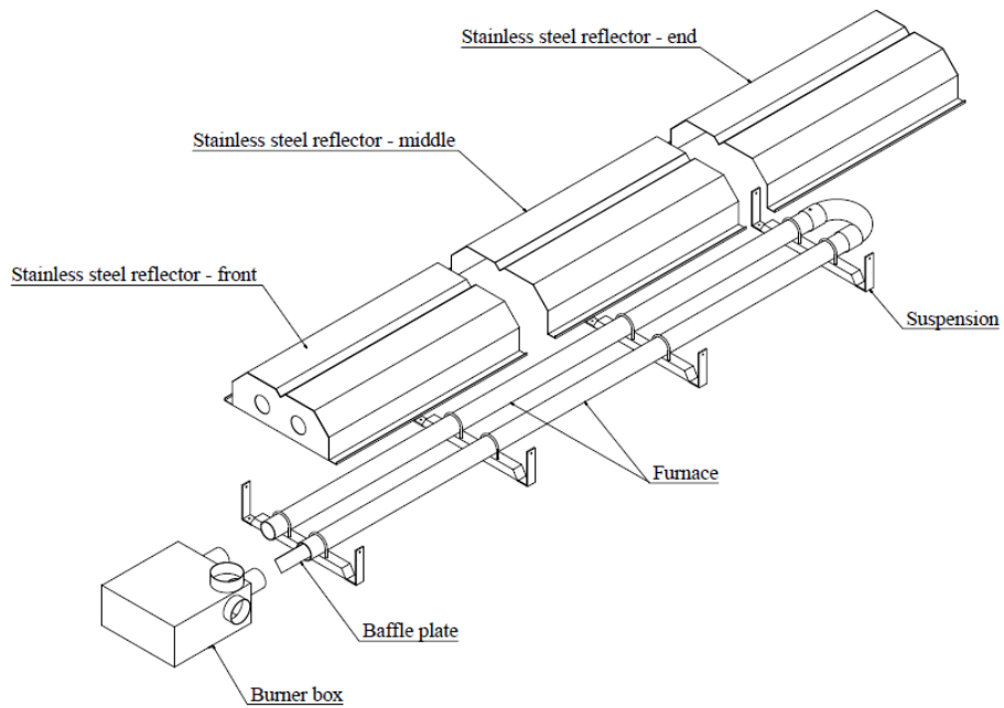
Fig. 1 Infrared heater KM-U with length from 3 to 6 m
