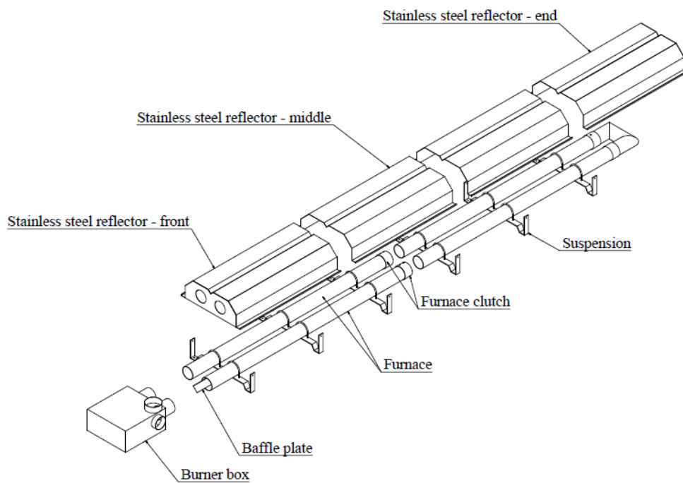
Fig. 2 Infrared heater KM-U with length 8 and 9 m
